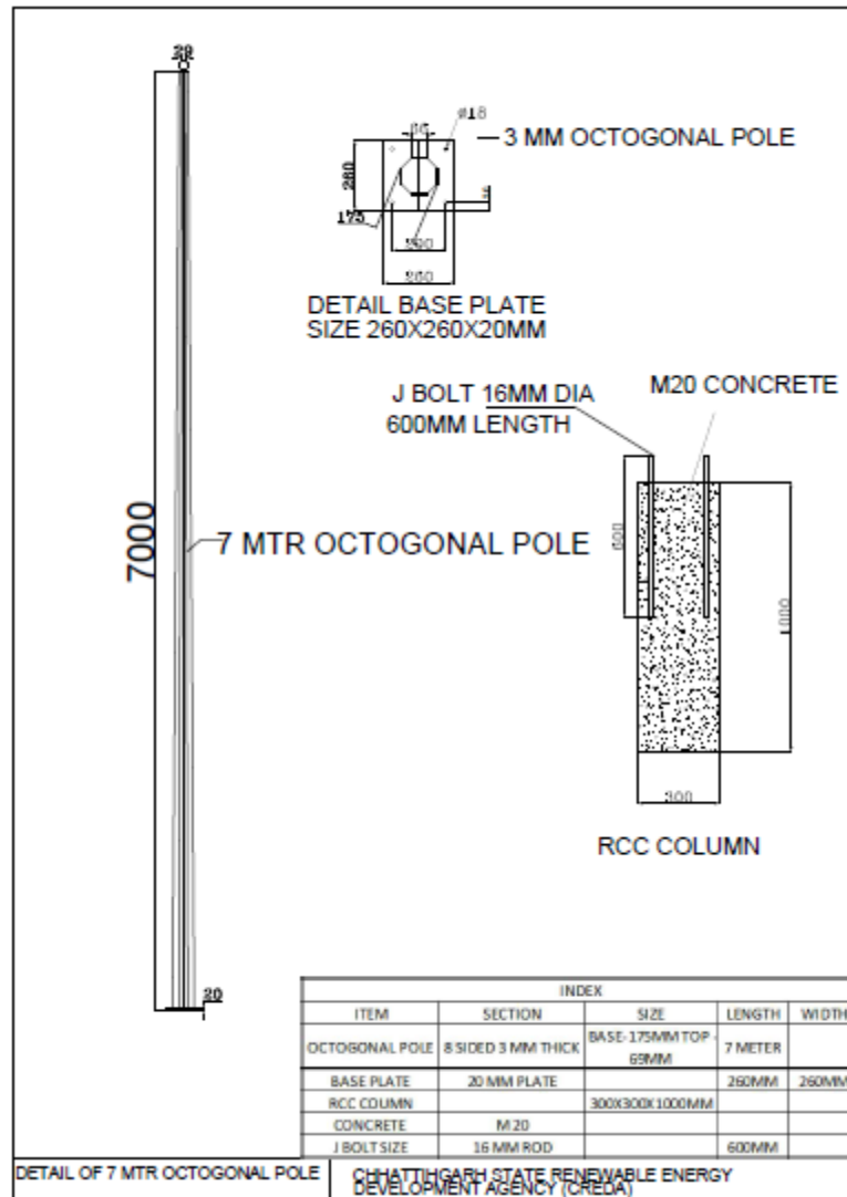
07 Mtr Pole Drawing
