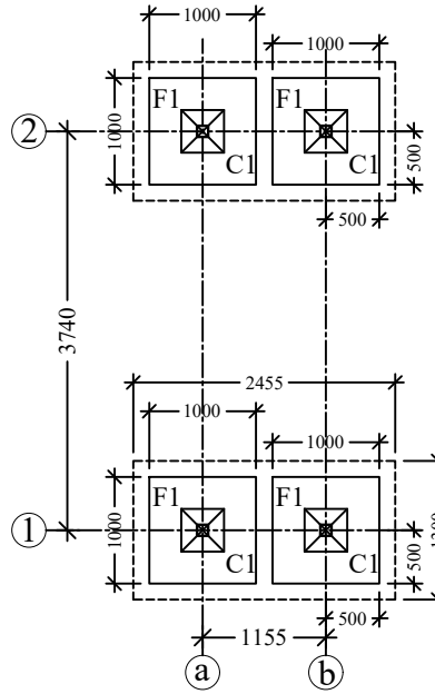
FOOTING CENTERLINE PLAN
