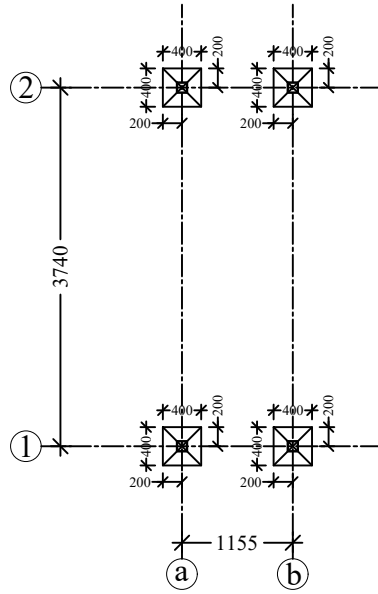
COLUMN CENTERLINE PLAN
