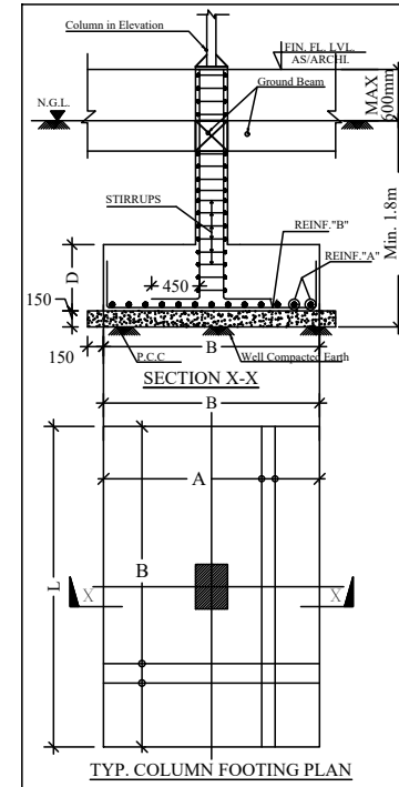
TYP. COLUMN FOOTING PLAN
