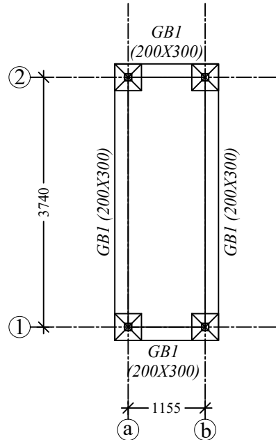
GROUND BEAM PLAN
