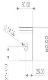
U-CLAMP (160X50X5)
